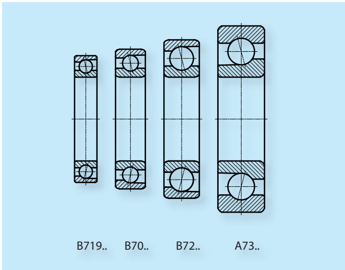
Fig. 1.2. Series of high-speed spindle bearings
