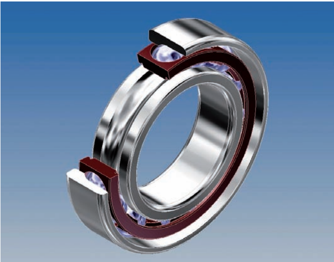
Fig. 1.1. Spindle bearing
