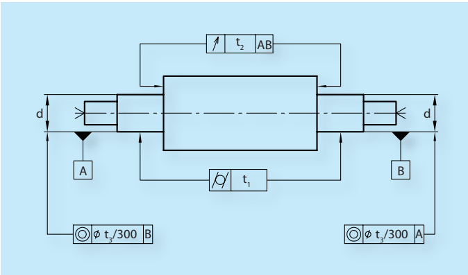
Fig. 17.1. Machining of cylindrical shafts
