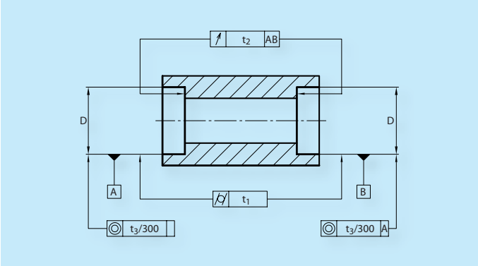
Abb. 17.4. Machining of housing bores
