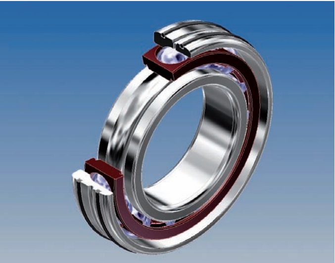
Fig. 6.1. Spindle bearing in DLR design
