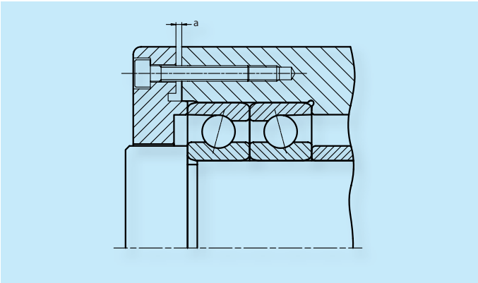
Fig. 9.1. Fastening with housing cover
