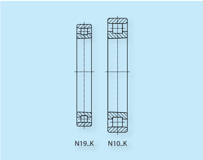
Fig. 13.2. series of single-row high-precision cylindrical roller bearing
